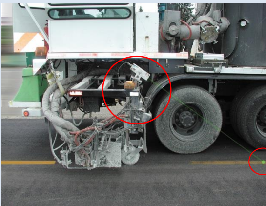
Gun Carriage Guidance - The laser is used to give the operator "heads up" time to move the gun carriage in and out for easy and precise alignment.
